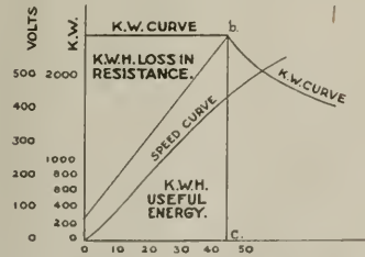
FIG. 2—ENERGY RESISTANCE LOSS.
